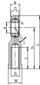
Type SIZP...S
