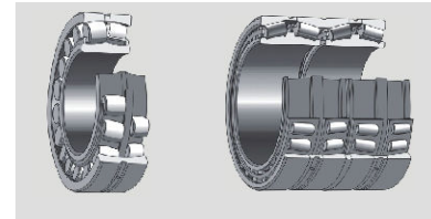
Double-row Bearing Fig1. 4. 15
