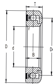
Type RTM
