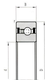
Type TD...2RS
