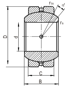
Type GEFZ...S
