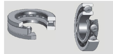
Thrust Roller Bearing Fig1. 4. 13
