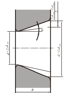
Fig 8.5 Tapered bore with actual diameters and their deviations
